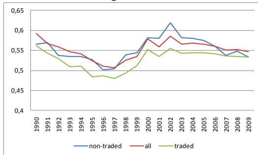
Figure 6: SD
