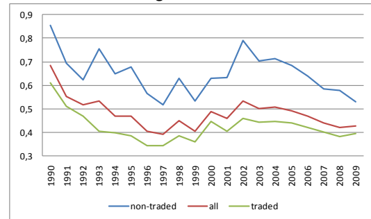
Figure 7: MSE
