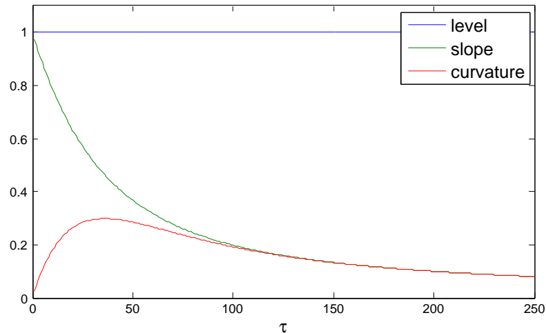
Figure 4.1: Factor Loadings
