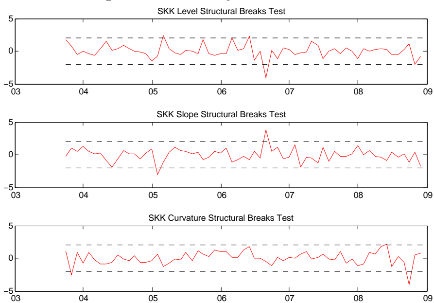
Figure A.5: Auxiliary Residuals – SKK
