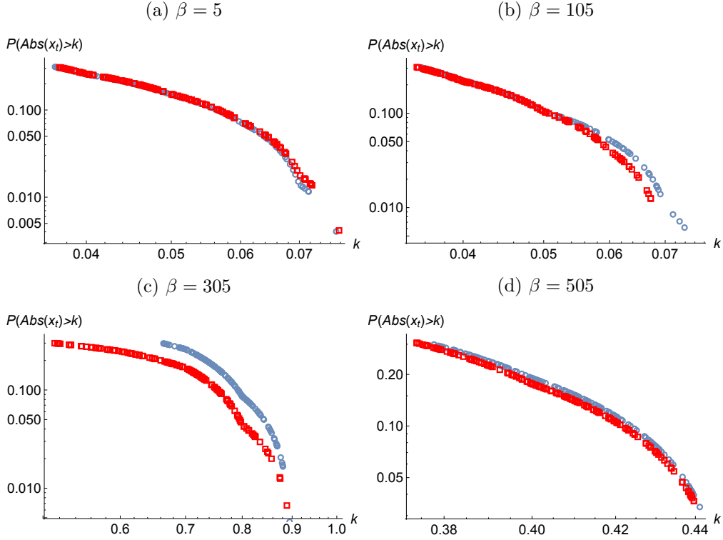
Figure 3: Plots of the tails of sample x_t time series' empirical distributions with the PT feature (red squares) and without it (blue circles).
