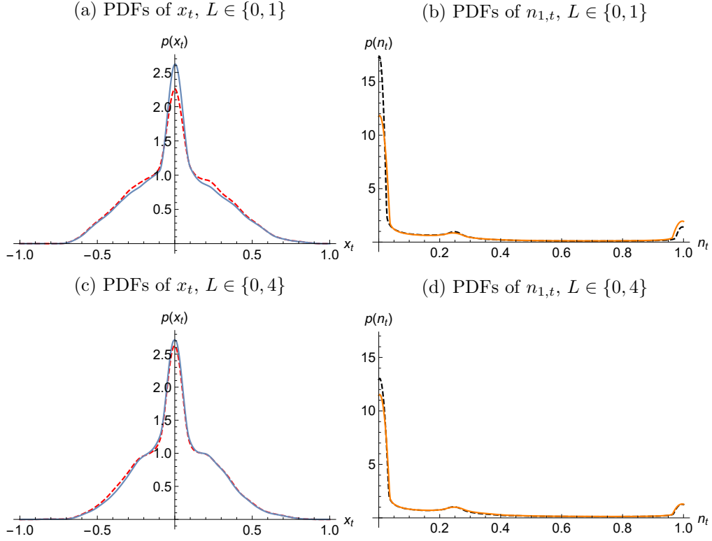
Figure 4: Behavior of the model for different L versus the benchmark case of L = 0 (depicted by dashed lines), \beta = 405 and K = 15 .
