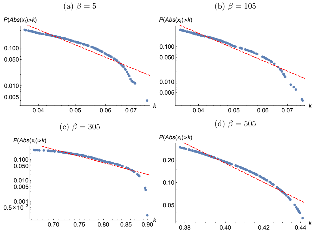
Figure 6: Plots of the tails of sample x_t time series' empirical distributions and OLS fit. Benchmark case without the PT feature.
