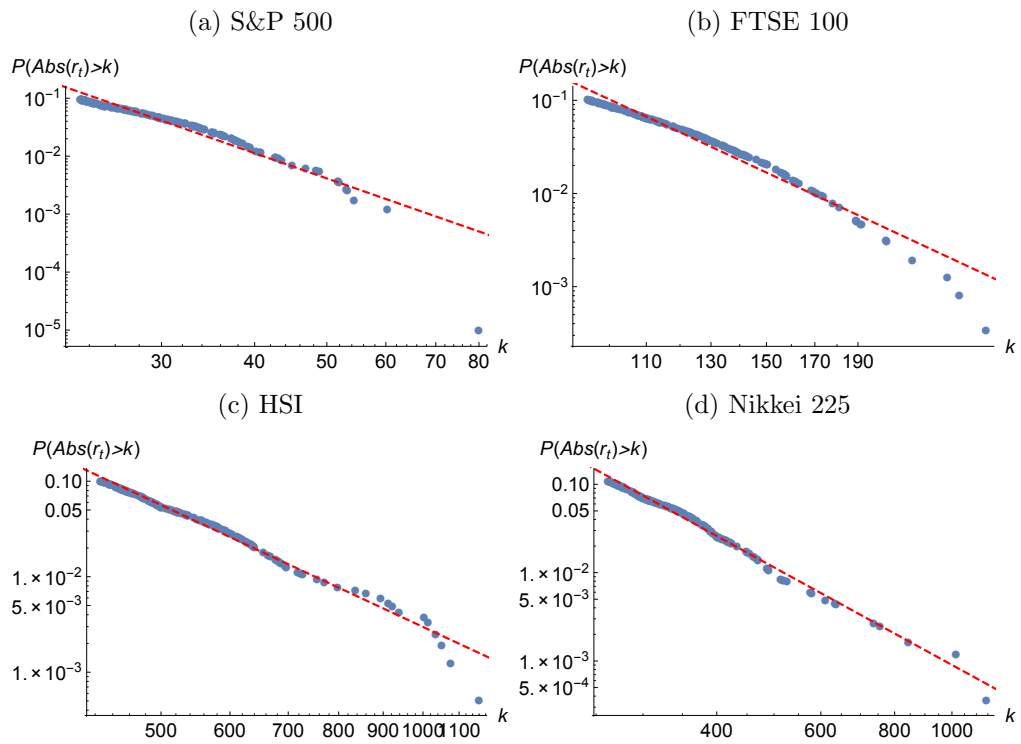
Figure 9: Tails of real stock market indices close price differences distributions; log-log scale; data retrieved from Yahoo Finance.
