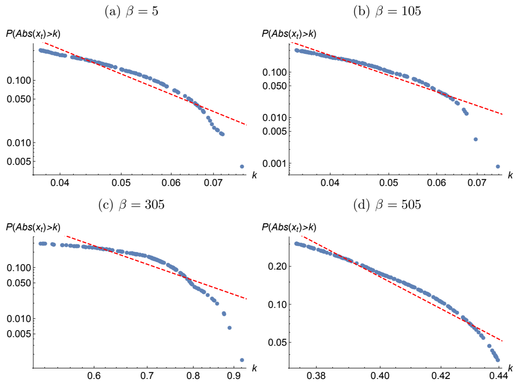
Figure 7: Plots of the tails of sample x_t time series' empirical distributions with the PT feature employed and OLS fit.
